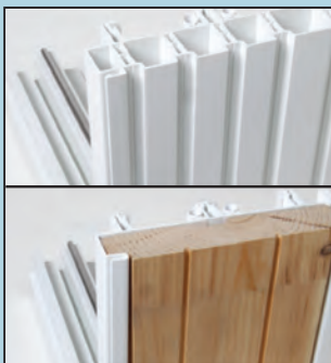
All Vinyl Frame (Top) Vinylclad Wood Frame (Bottom)
